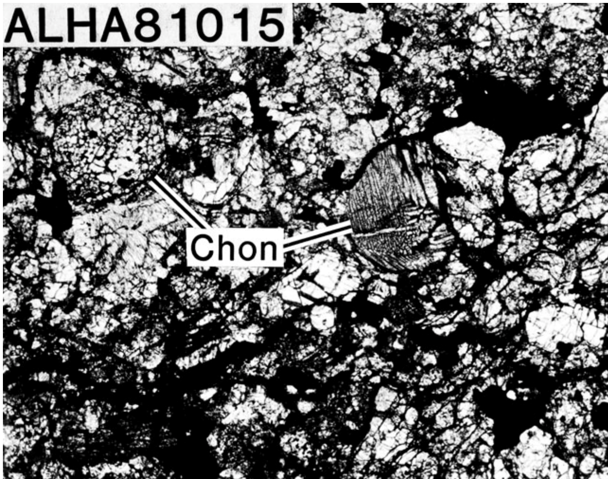
Figure 10: Petrographic thin section image of ALH A81015 illustrating the texture of a thermally metamorphosed chondrite with chondrules starting to have more diffuse boundaries compared to those in
